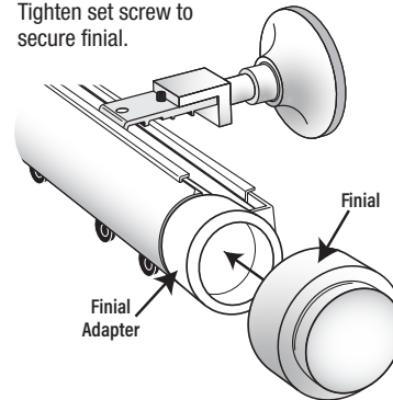
Finials for Metro Flat Fascia Slide finial onto rod. Tighten set screw to secure finial.
